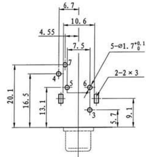
PCB LAYOUT
